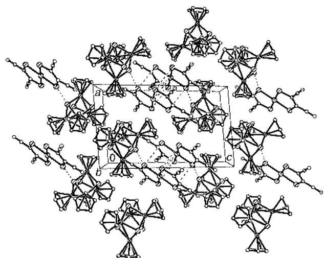
Fig. 4 The crystal structure of complex 5 as viewed along the b axis.
